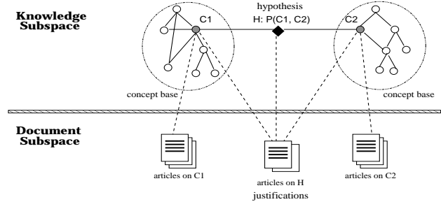
Figure 2: A DL information space for high-order cognition support
