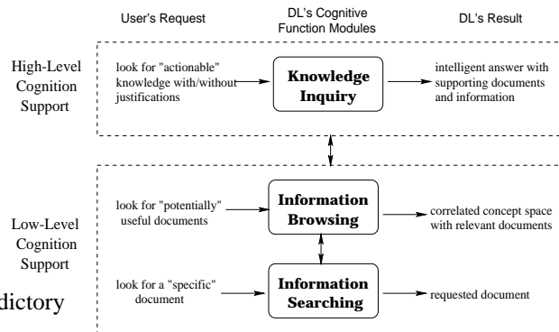
Figure 1: A two-layered DL cognitive function model
